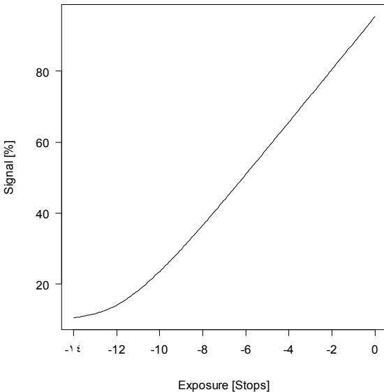
Figure 1: Log C curve used in ALEXA SUP 3.x
