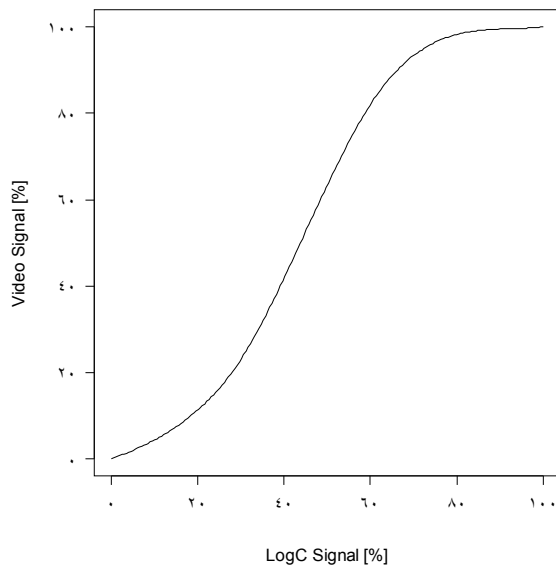
Figure 2: Tone-map curve (including video gamma correction)
